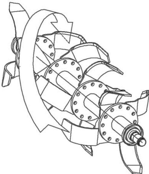
Figure 4-8 Helical Arrangement
